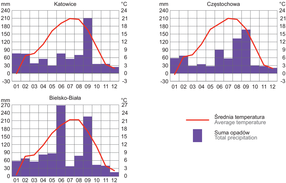
CHART 1. AIR TEMPERATURES AND PRECIPITATION AT SELECTED METEOROLOGICAL STATIONS IN 2024
