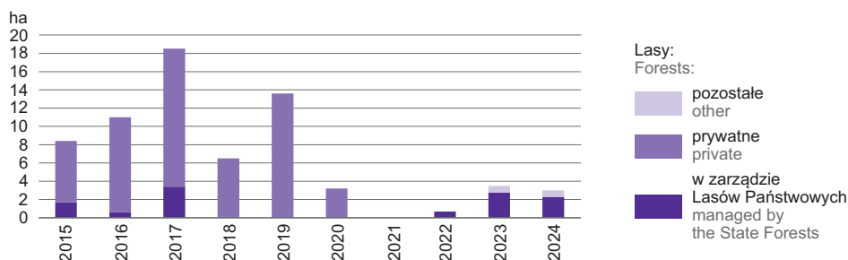
CHART 3 (74). AFFORESTATION a
